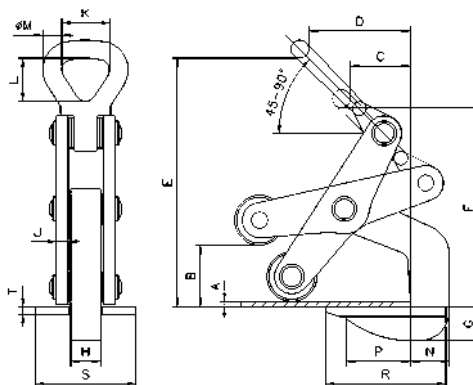
TWL with roller
