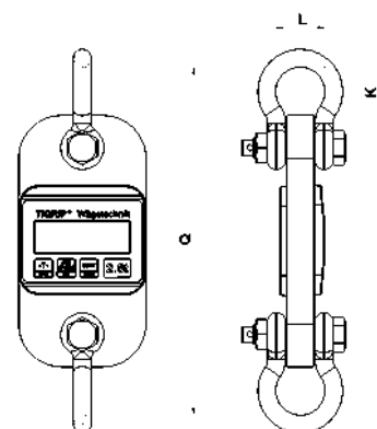
Load indicator TZL/TZR with shackle
