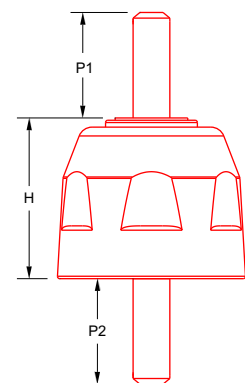
Male-Male Combination
