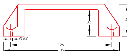
NYLON HANDLE NH 40145
