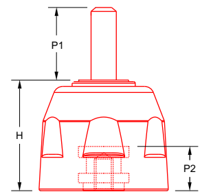
Male-Female Combination
