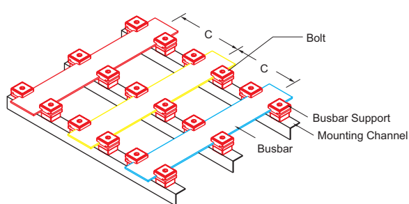
Single Busbar Fixing Arrangement C-C = Centre to Centre Phase distance in mm
