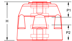
Female-Female Combination
